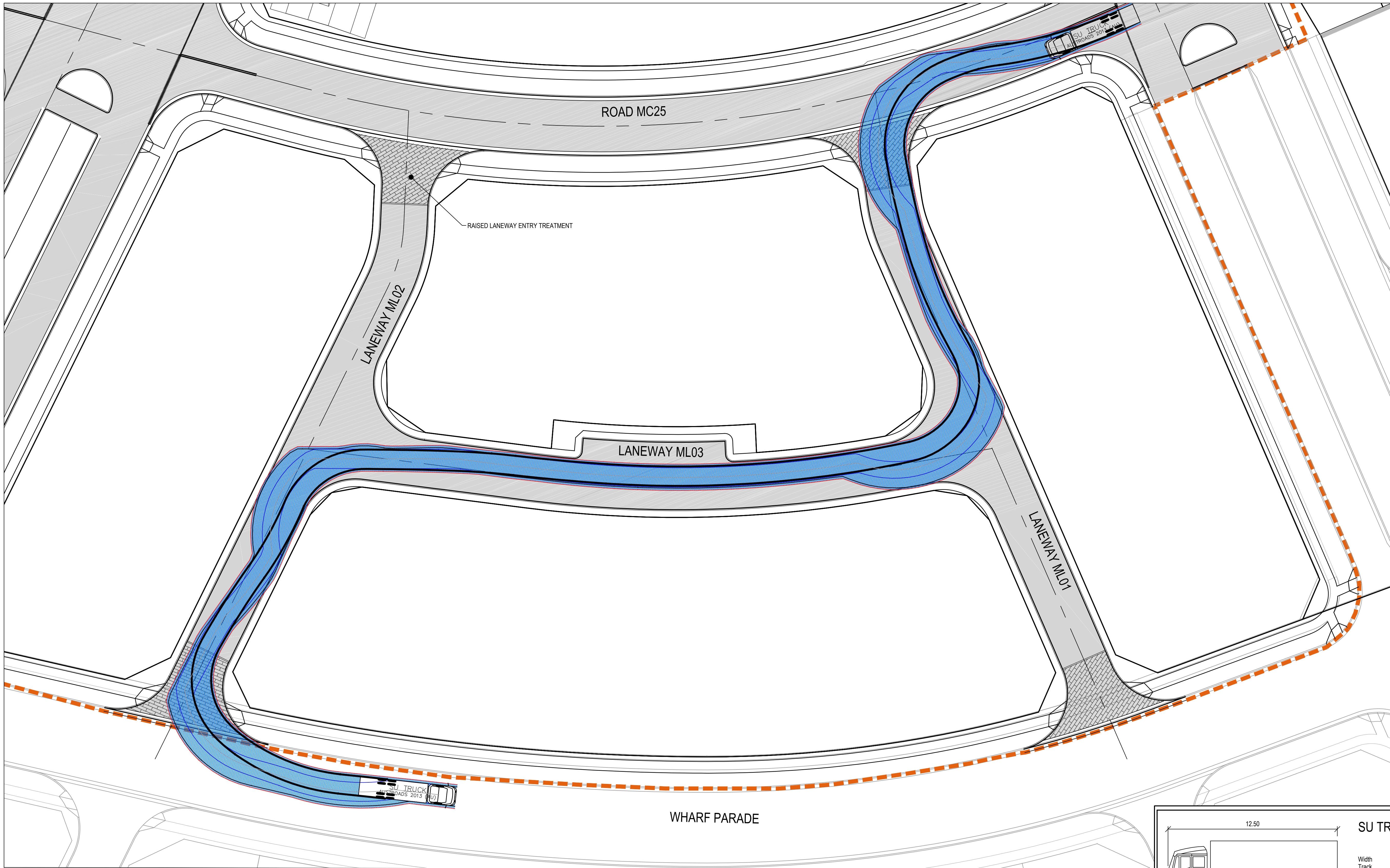
ROAD ML01 - ML03 - ML02 GARBAGE TRUCK SWEEP PATH SCALE 1 : 250
